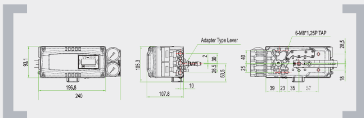
YT-3350R
